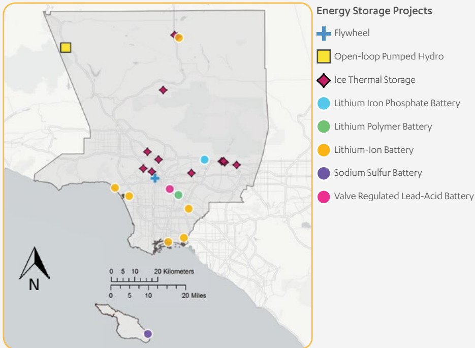
Energy Storage Projects in LA County as of January 2017
