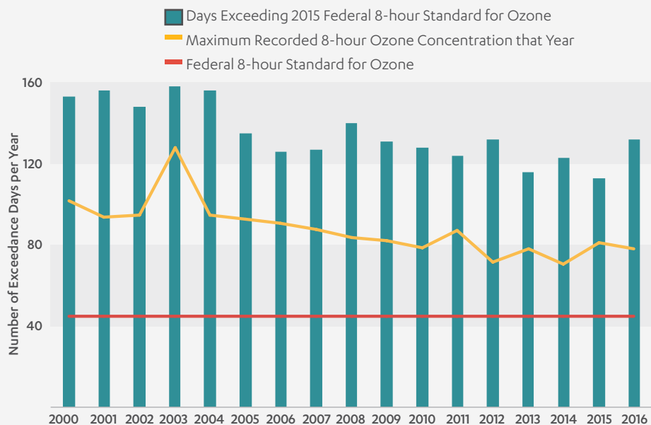
South Coast Air Basin Ozone Trends (2000-2016)
